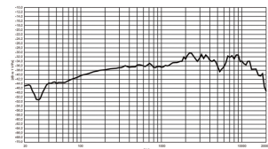
GF-923 Frequency Response
