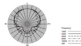
GF-923 Polar Pattern
