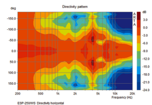
ESP-250WS Directivity horizontal
