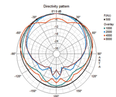
ESP-250WS Directivity horizontal
