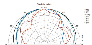
EDL157WS Directivity horizontal
