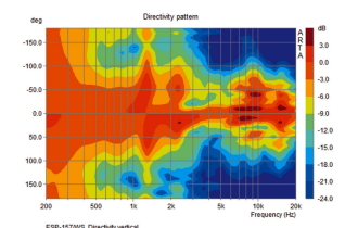
ESP-157WS Directivity vertical
