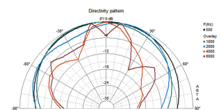
ESP-157WS Directivity vertical
