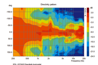
EDL157WS Directivity horizontal
